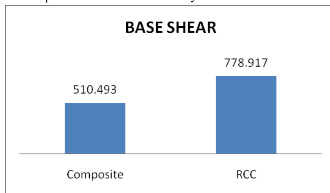
Graph 6 Base Shear Comparison
